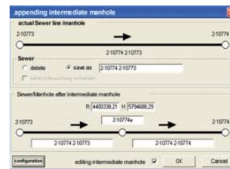
IBAK IKIS appending an intermediate manhole
