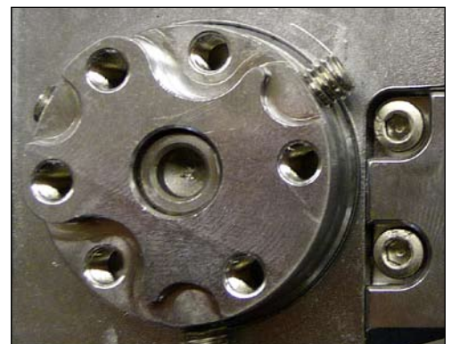
Afterwards, the wheel adapter is screwed on. It is possible to mount all T66 wheel sets onto this.
